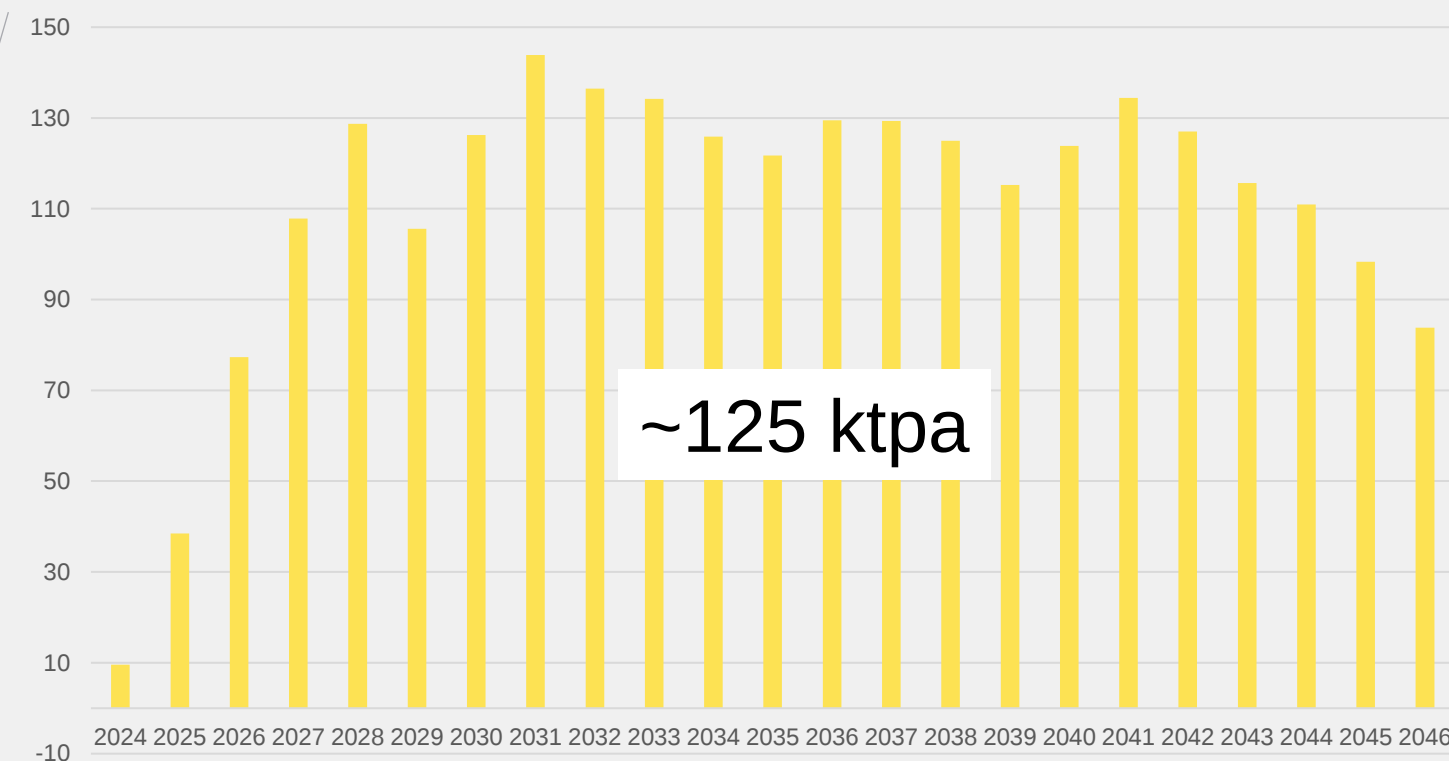
Nickel, kt
