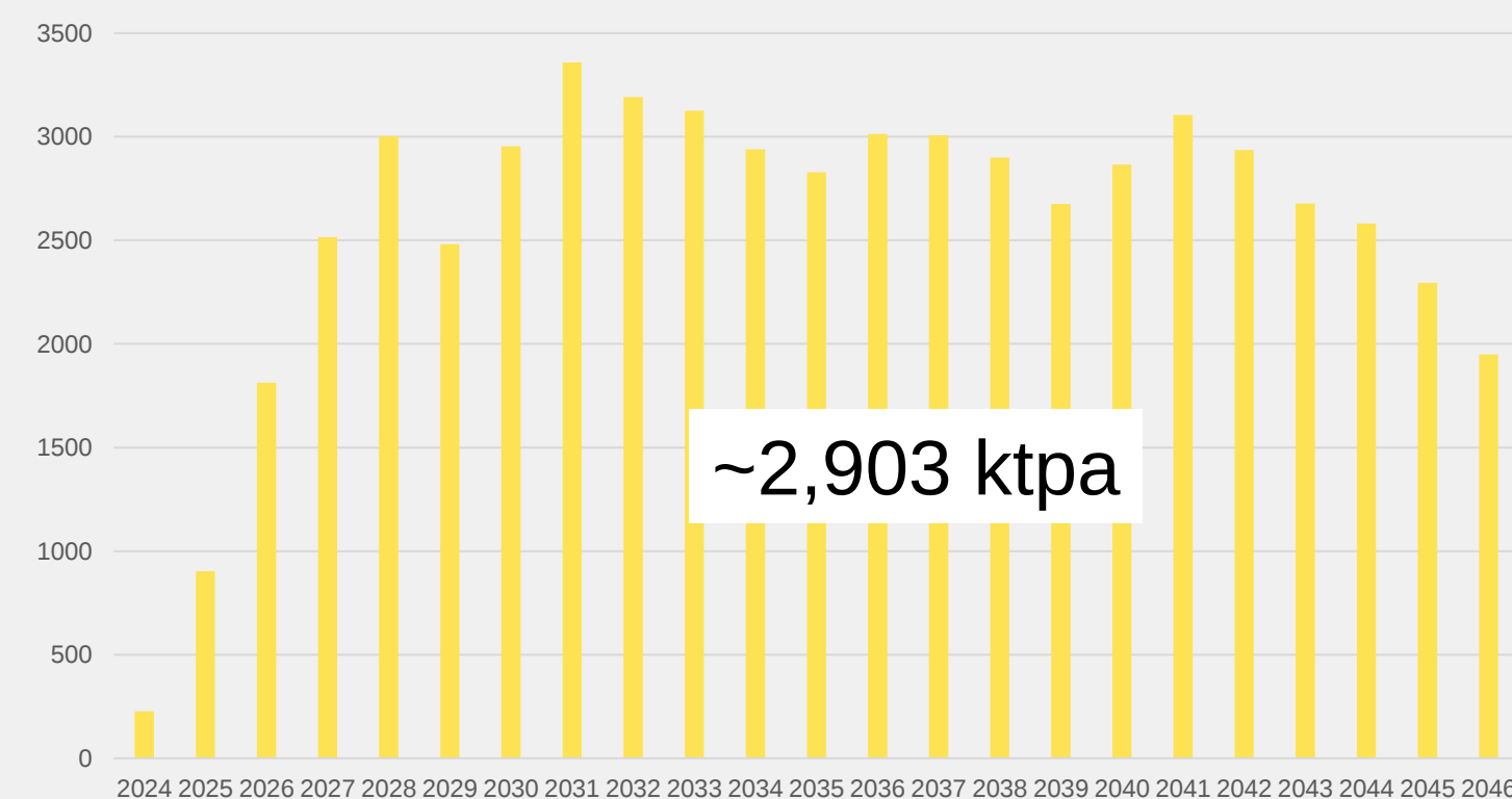
Manganese, kt
