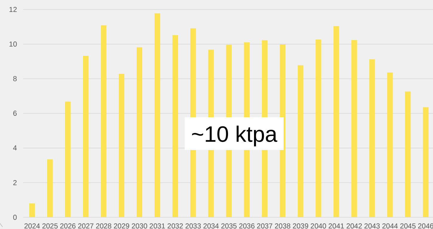
Cobalt, kt
