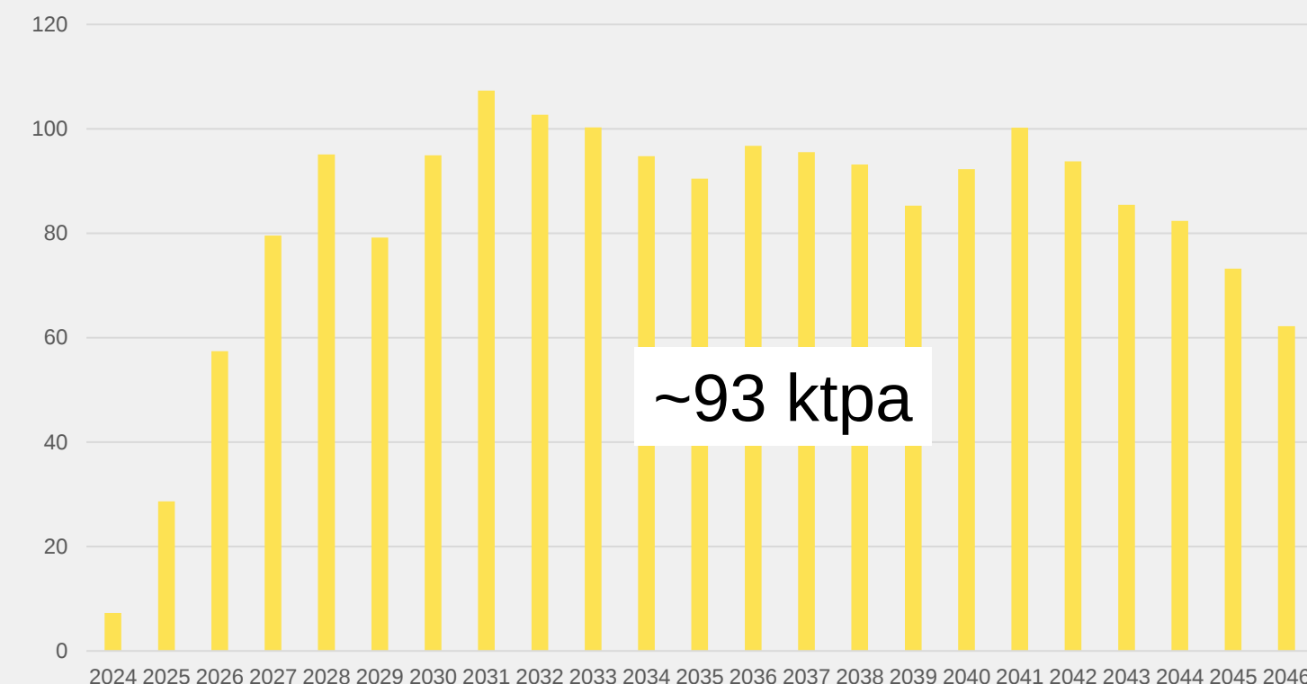
Copper, kt
